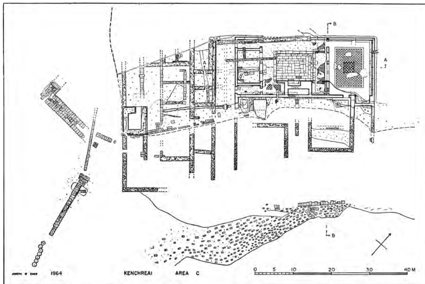
Plan 2, Northeast End of Harbor ( Area C ). Actual State
