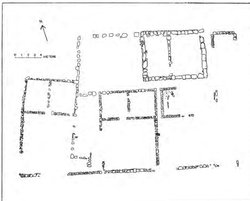
Plan 2. Perachora. House and Temple foundations
