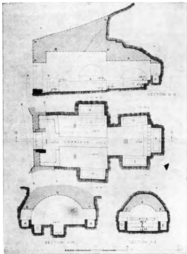
Corinth. Early Roman Painted Tomb: a. Plan and sections, b. East Wall of Corridor, North Half, c. East Wall of Corridor, South Half
