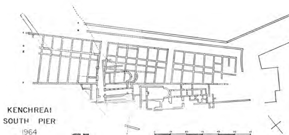
Plan 3. Southwest End of Harbor. Generalised and incomplete
