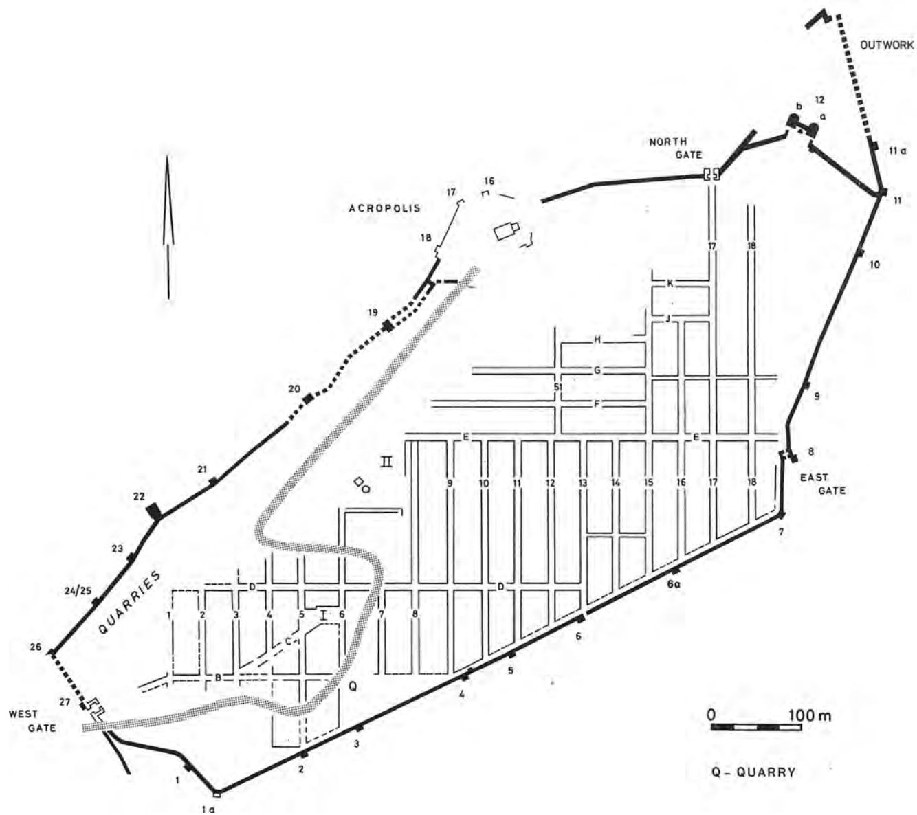
Fig. 1. The Goritsa Fortress near Volos. General Plan.
