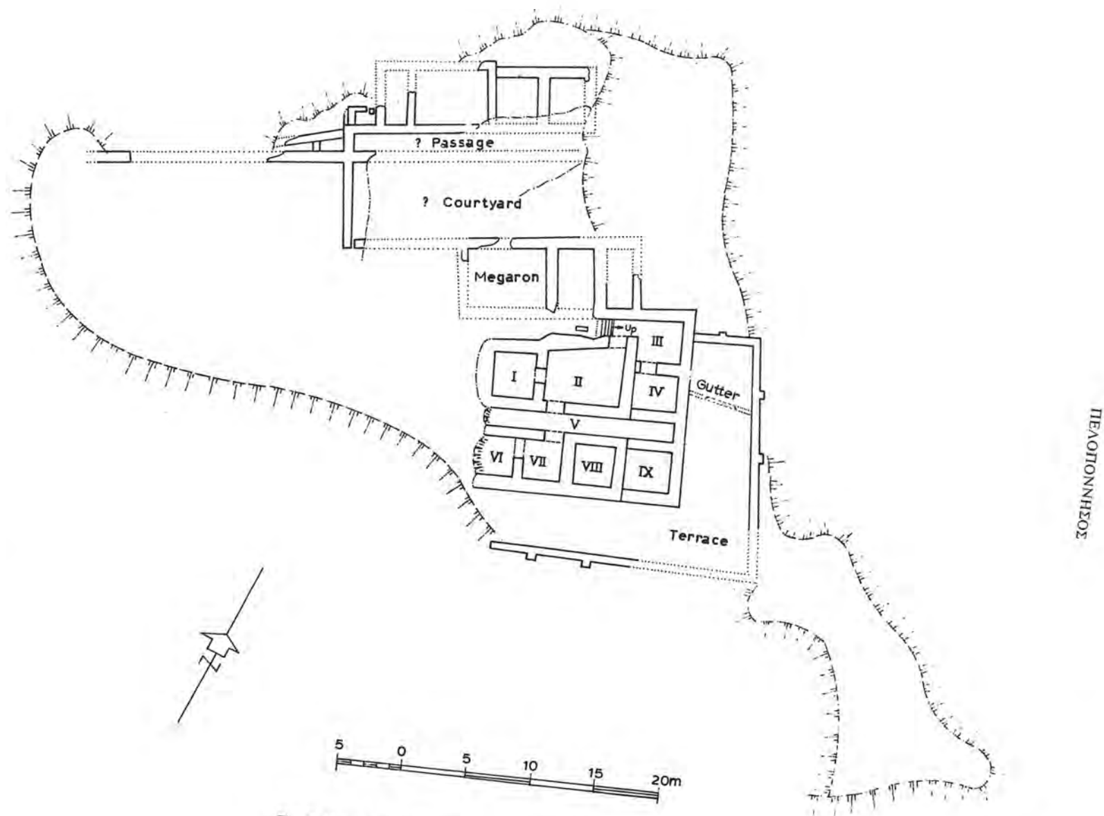
Fig. 3. Menelaion. Plan of Mycenaean buildings. Period II.
