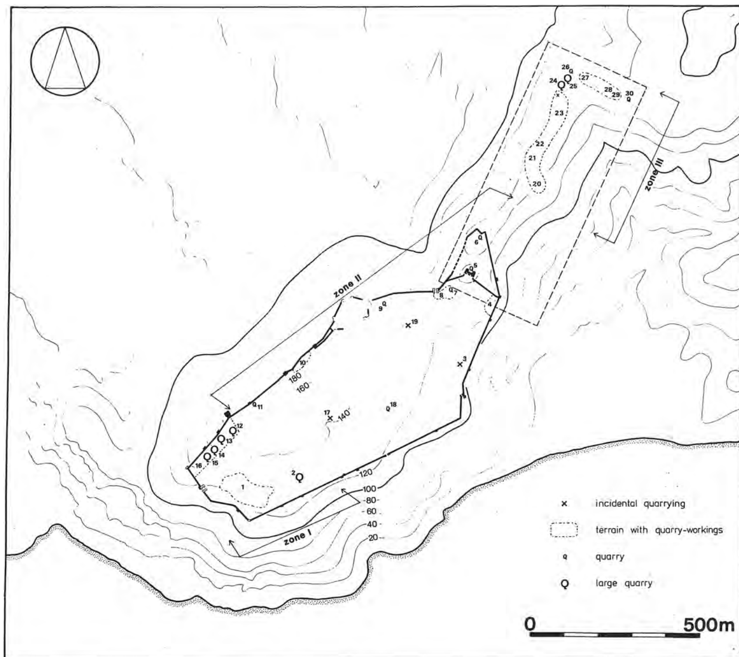
Fig. 4. The Goritsa. Foztress near Volos. Survey of the quarrying areas.
