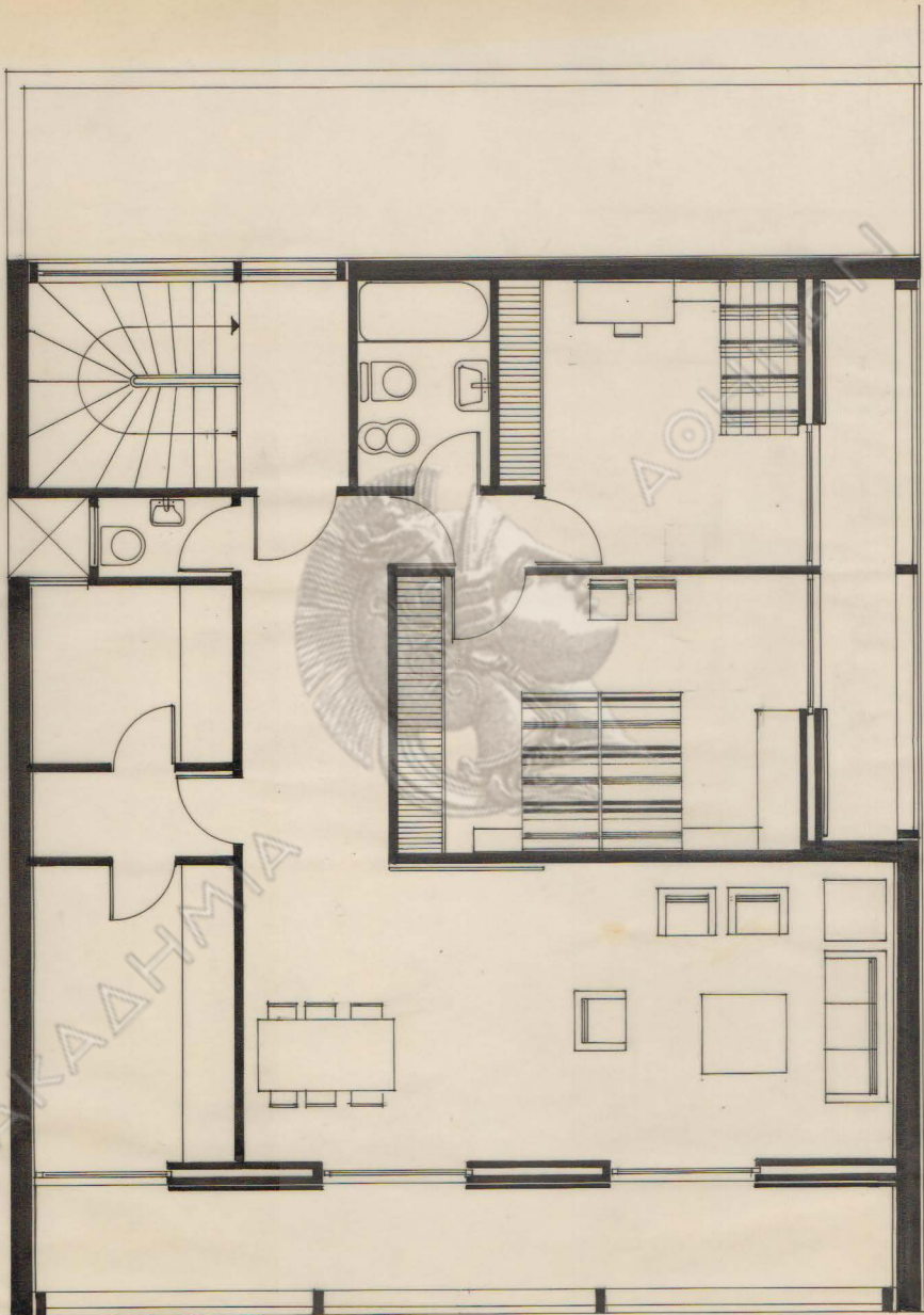
ΚΑΤΟΨΙΣ ΟΡΟΦΟΥ
